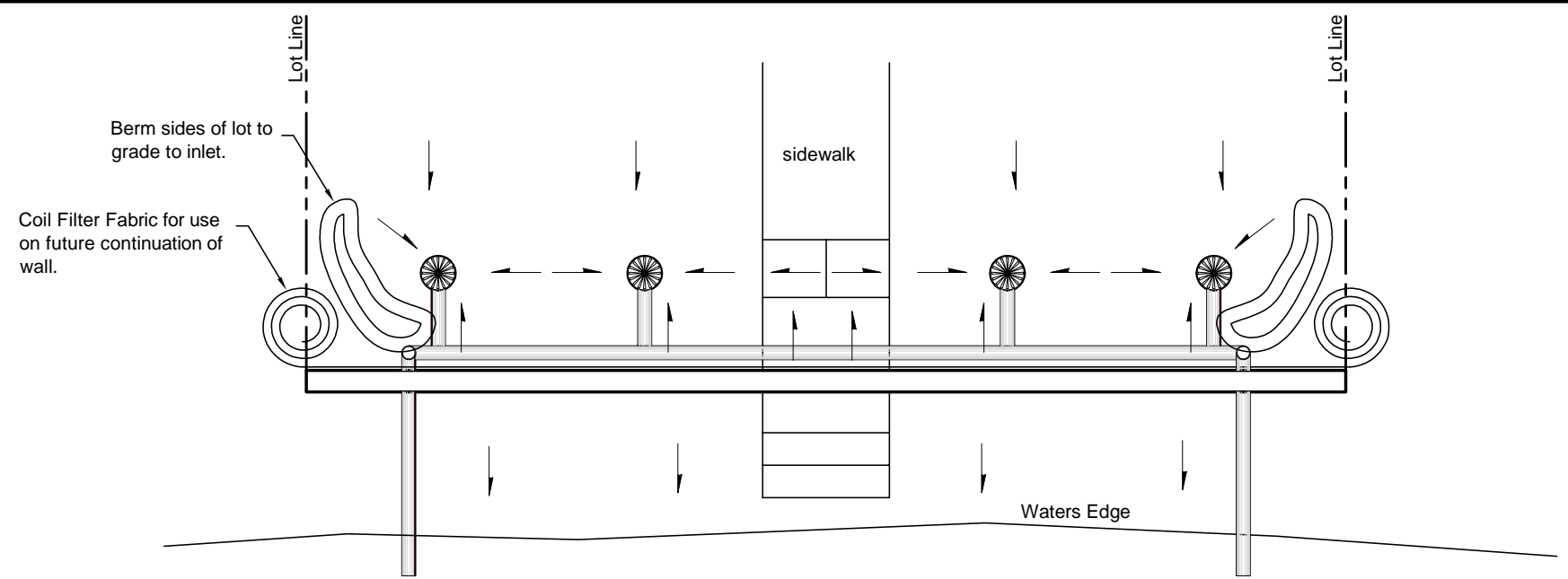
Plan View of Wall
