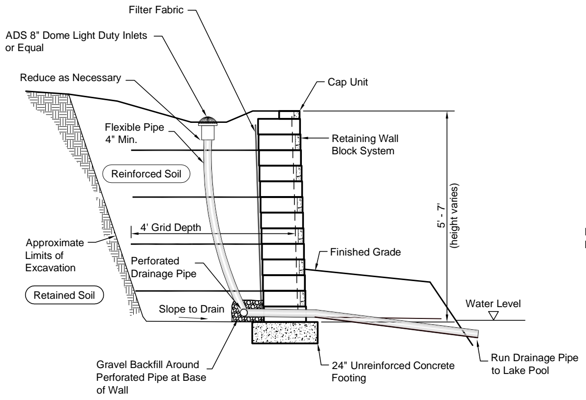
Wall Section Using Retaining Block System
